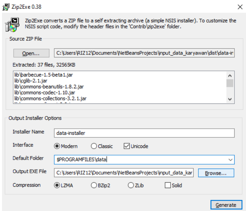
Gambar 88. Pengaturan Installer Zip
