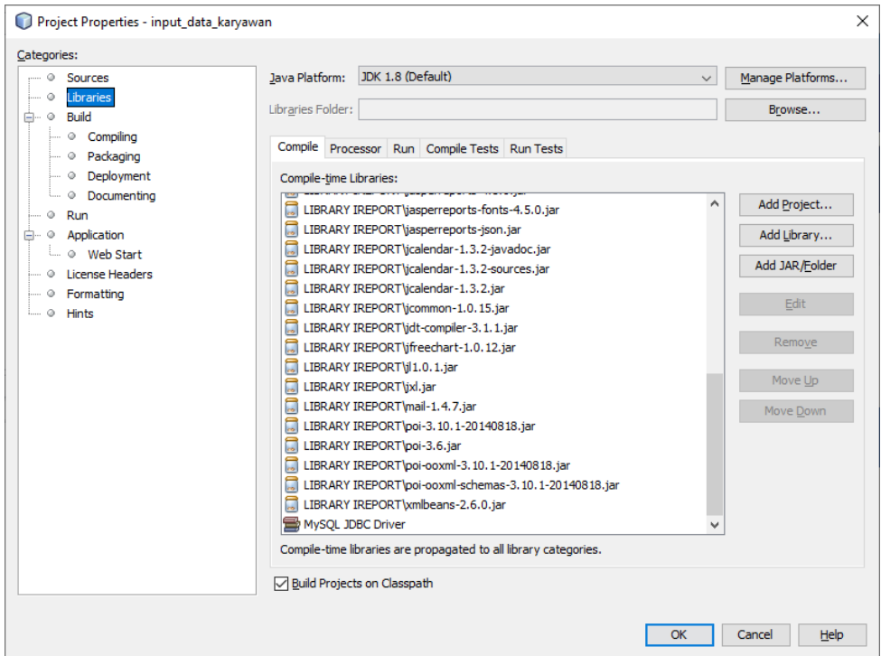
Gambar 73. Isi Compile Libraries
